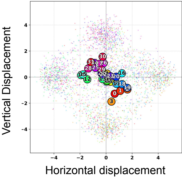
humanoidmaze-medium-navigate-v0 (K=32, L=80)
