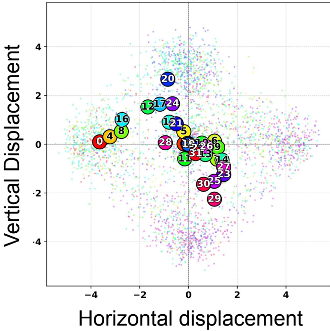
humanoidmaze-medium-navigate-v0 (K=32, L=80)
