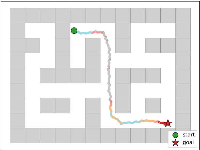
D-GCIQL antmaze-large-navigate-v0 (task 3)
